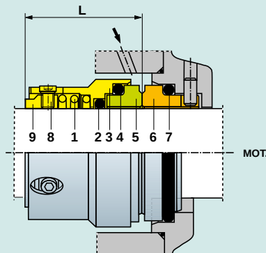
TYPE 85M with cylindrical spring Also available TR CL
