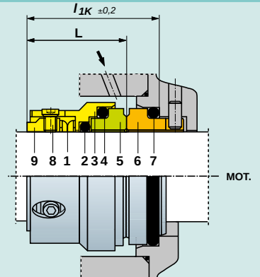
TYPE 85N with sinusoidal wave spring Also available TR CL
