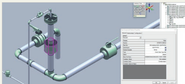
Smart 3D valve based on GF Piping System parts
