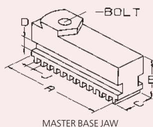
MASTER BASE JAW
