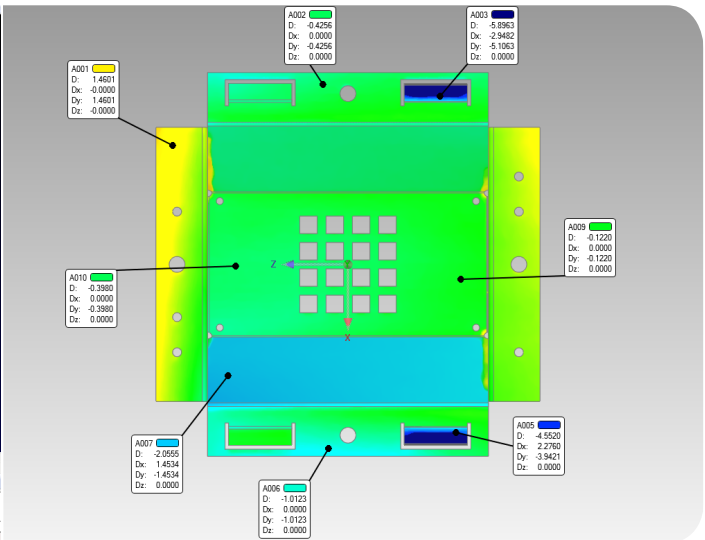
Figure 5: Comparison of scan to 3D CAD model
