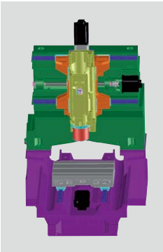
Thermally symmetric structure Equal left-right construction permits straightforward thermal distortion
