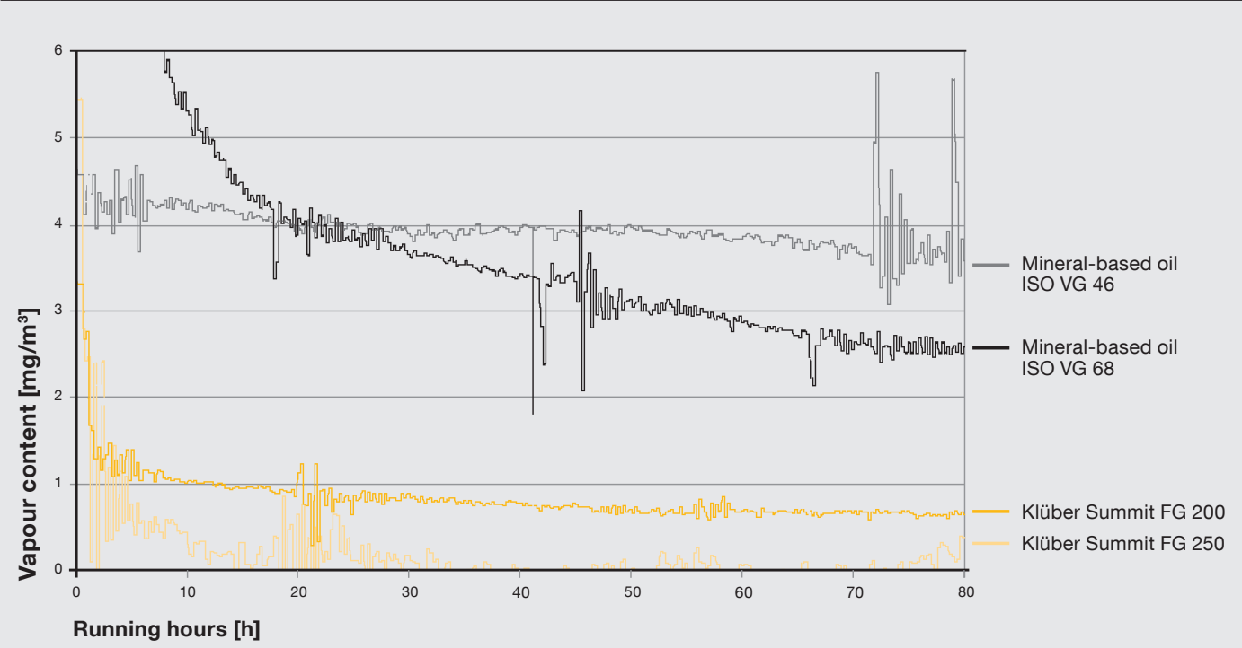
Oil content in the compressed air at 100 °C [mg/m³]
