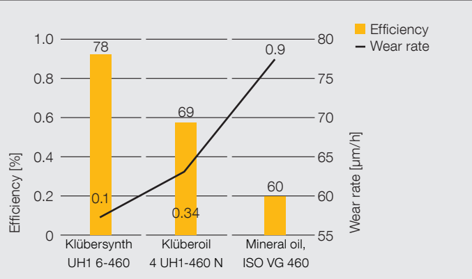
Efficiency determined on the Klüber Lubrication worm gear test rig
