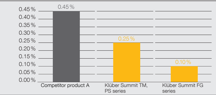
Conradson Carbon Residue* Test, percentage
