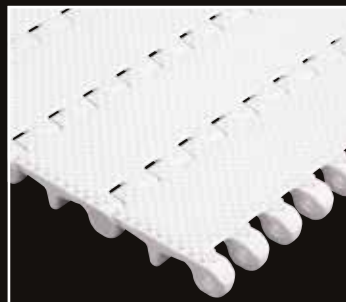
50-838 Closed nub top surface for minimum contact between belt and candy, EASY TO CLEAN for sticky products
