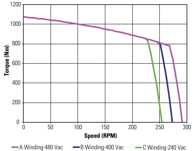
KBM(S)-163X02 ContinuousTorque
