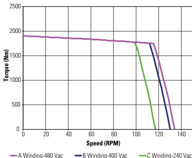
KBM(S)-260X01 ContinuousTorque
