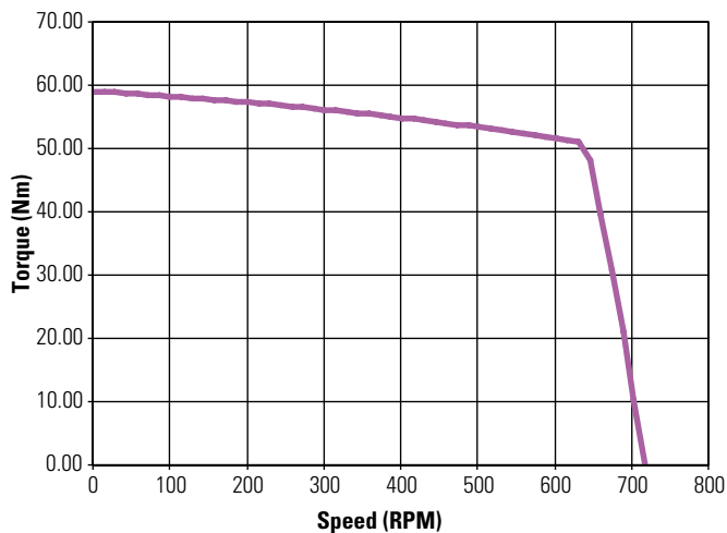
KBM(S)-57X03 ContinuousTorque
