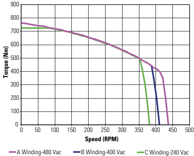
KBM(S)-163X01 ContinuousTorque
