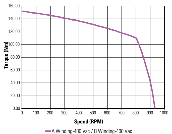
KBM(S)-60X03 ContinuousTorque
