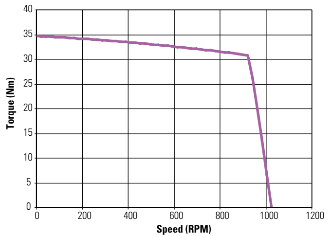
KBM(S)-43X04 ContinuousTorque
