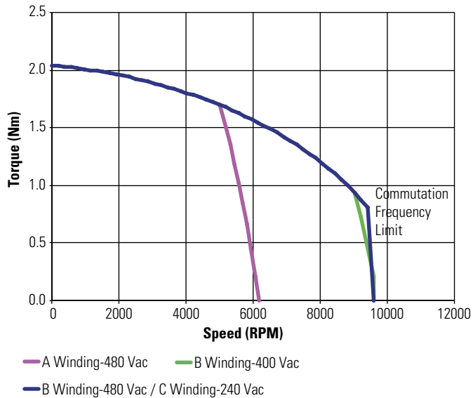
KBM(S)-17X01 ContinuousTorque
