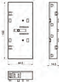
Auxiliary contact
