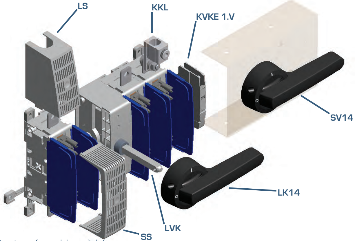
Structure of a modular switch fuse
