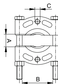
External puller UEE
