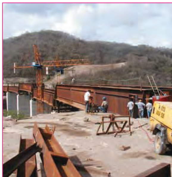
Construction of "Sistema de Transporte de la Región Central de Venezuela, Primera Etapa Caracas Tuy-Medio" through the development of railway viaducts with metallic floor systems lowered with EUROPRESS hydraulic equipment (Caracas, Venezuela June 2003)
