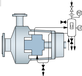
Plan 53A
