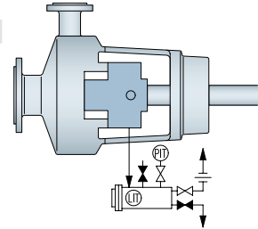
Plan 75
