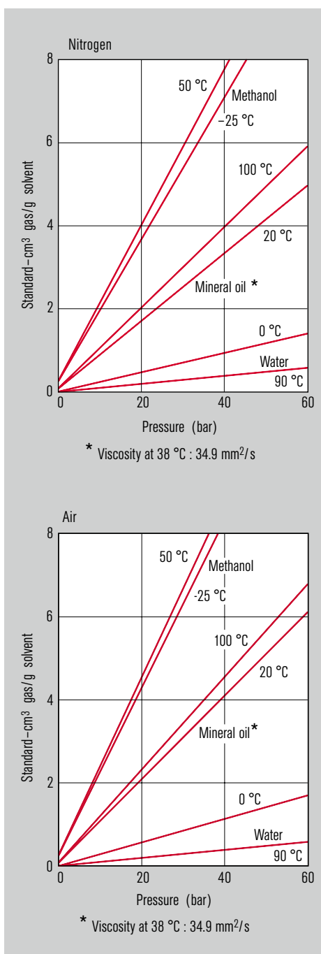
Gas solubility in typical barrier media
