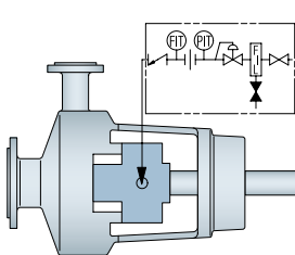
Plan 72
