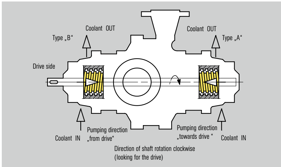
Contra-rotating pumping screw.
