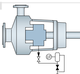
Plan 65B
