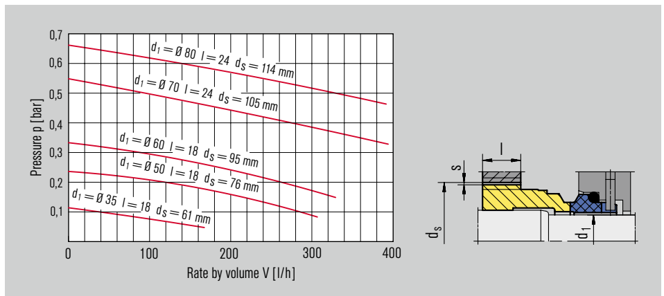
Pumping capacity of various pumping screws without pumping sleeve
