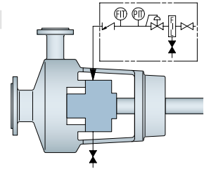
Plan 74
