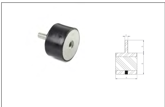
AAG vibrationsdæmper Type B
