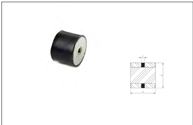
AAG vibrationsdæmper Type C
