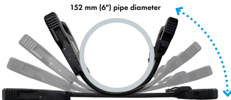
The D-DR 1025B NDT and the D-DR 1043B NDT can be bent continuously from flat to a 152 mm diameter in one direction.
