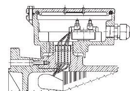
Frame size 63–112
