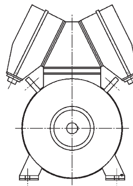
Motor with two HV boxes
