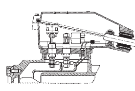
Frame size 250–450 Frame size 250 and 280 with with connection plate as for 180–280
