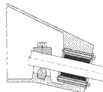
Version 9 Split terminal box with internal strain relief clamp, cable entry according to EN 50019
