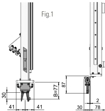
Standard version with sprue gripper
