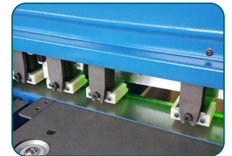
Specially-designed rectangular hold-downs, suitable for cutting narrow stripes (optional)
