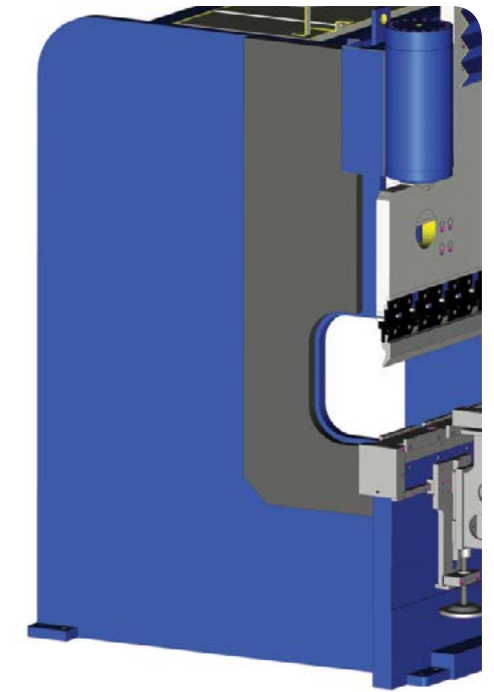
Extra external welded-steel side frame to increase machine's rigidity and minimize deformation.
