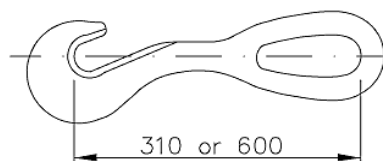
EXTENSION ROD HOOK
