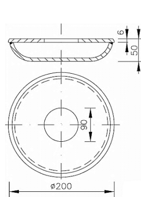
FLUSH CAR LASHING
