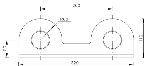
DOUBLE LASHING PLATE
