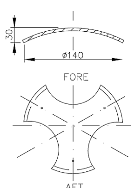
RAISED CAR LASHING
