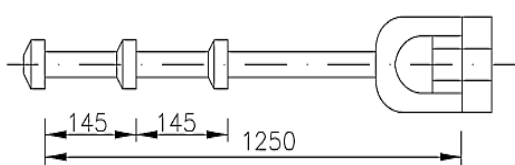
LARGE EXTENSION ROD
