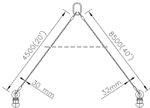
TOP LIFTING HOOK
