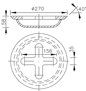
LARGE FLUSH
