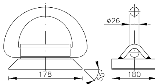
DOVETAIL 55°
