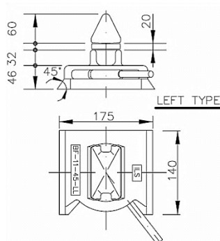
LINE LOAD 45°
