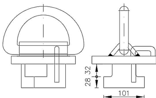
TURNFOOT
