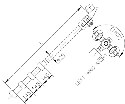
VERTICAL
