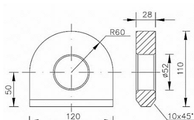
SINGLE LASHING PLATE
