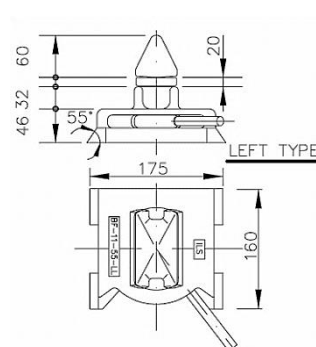
LINE LOAD 55°
