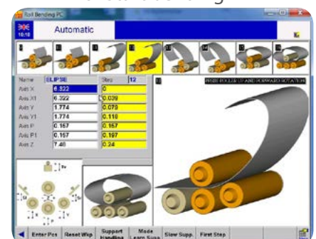
6- Start bending
