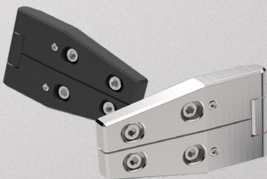
2 KLIMA-FLEX ADJUSTABLE 3D HINGE Specially designed hinges that ensure superb sealing properties. Available in stainless steel and zinc with metal or black texture coating.
