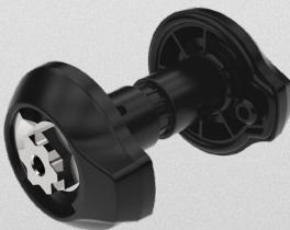
KLIMA-FLEX™ 2 LATCH UNIT Industrilas Klima-flex™ 2 has patented technology that allows for quick mounting in double-skinned doors. When you turn the screw, expanding legs are engaged and fix both door skins from the inside.
