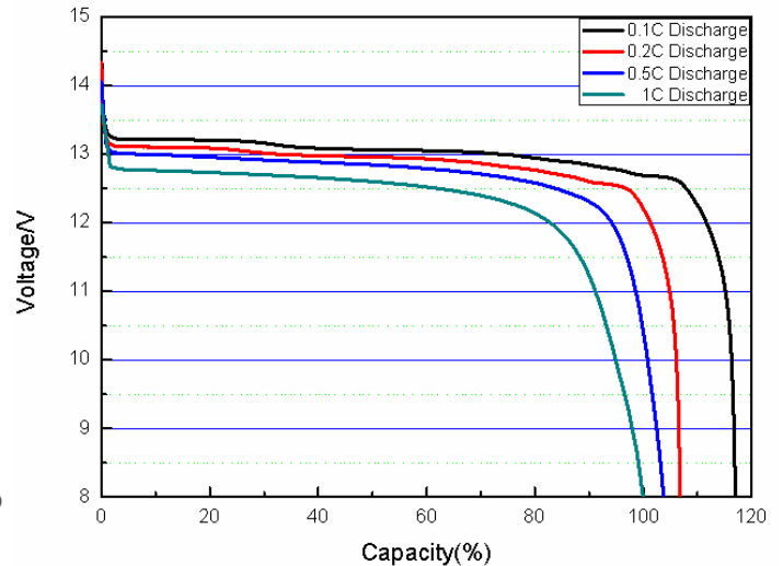
Discharge performance
