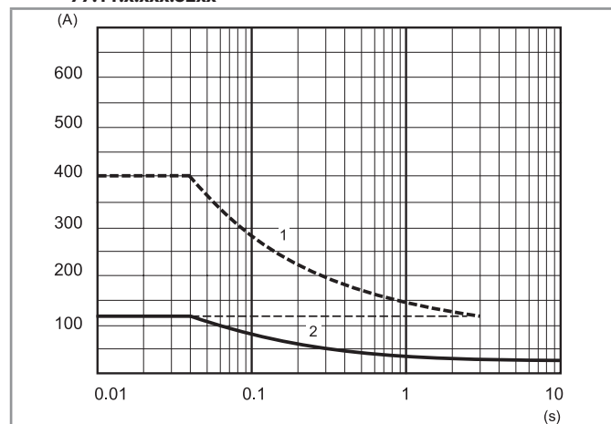
L77-11 Inrush peak current (AC) v inrush time 77x5.x.xxx.8x50
