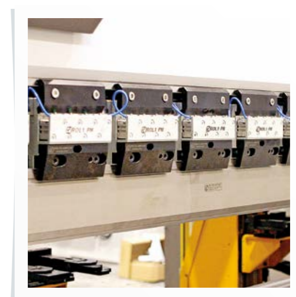
Pneumatic Tool Clamping System (O) Pneumatic tool clamping systems press and center the tools automatically with the help of the pressurized air. These are perfect solutions to shorten the setup timing and for automated press brakes.
