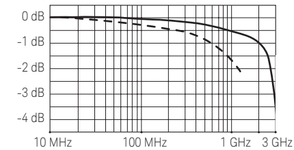
Insertion loss
