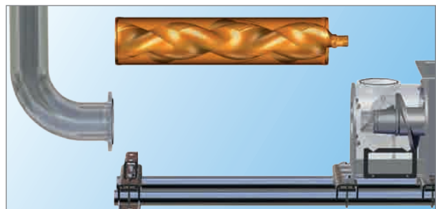
Step 3: Pull the stator and rotor along with the cardan shaft forwards and pull out of the pump housing.
