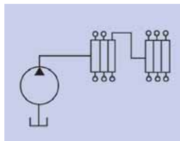
Schematic Progressive System
