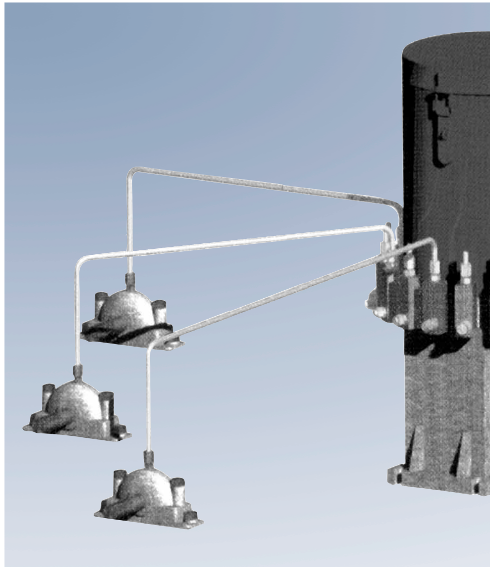
Schematic Combined Multi-line / Progressive System
