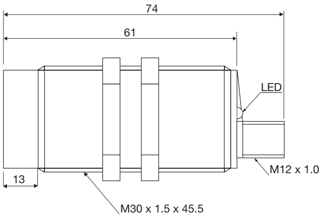
Fig. 9 Stik CA30CAN...M1IO
