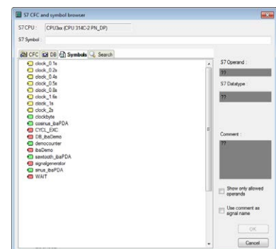
Convenient operand selection using a symbol browser
