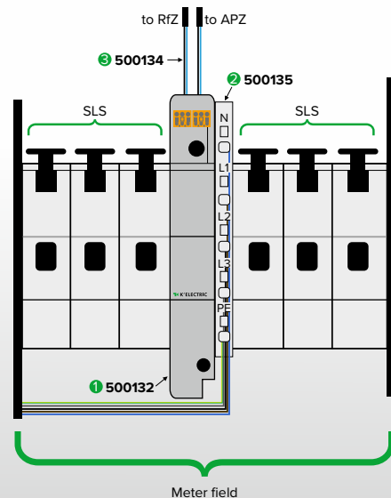
RfZ: Space for additional devices, APZ: Termination point meter location, SLS: Selective miniature circuit breaker
