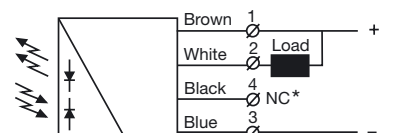
SPRR / SPPR / SPP / SPBS 26xx (load as NPN)
