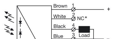
SPRR / SPPR / SPP / SPBS 26xx (load as PNP)
