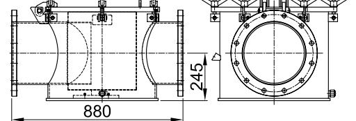
DN 300
