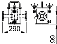
DN 25
