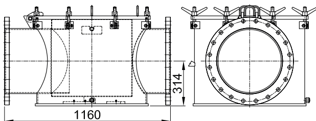
DN 450
