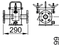
DN 40
