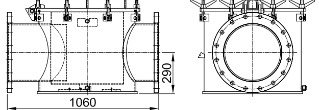
DN 400
