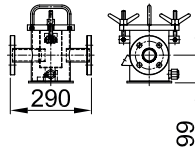
DN 32
