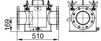
DN 150
