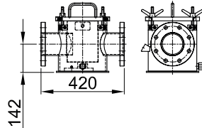
DN 100
