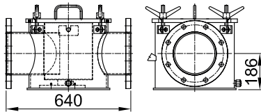
DN 200
