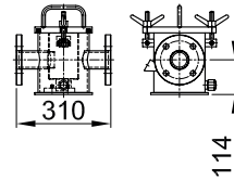
DN 50
