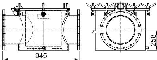
DN 350
