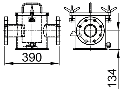
DN 80
