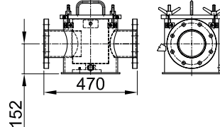
DN 125
