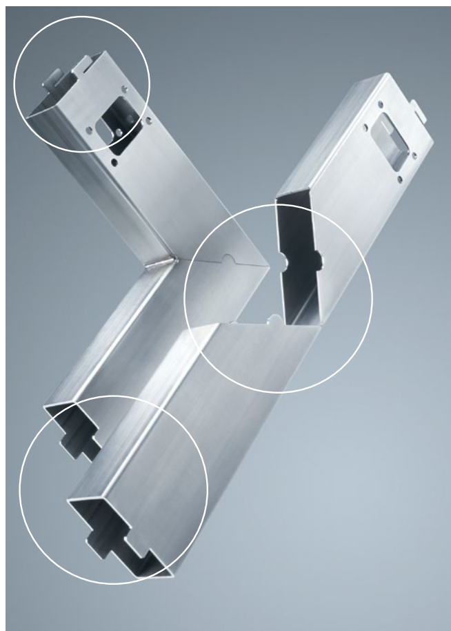
Efficient production of bend connections and positioning aids with a laser.
