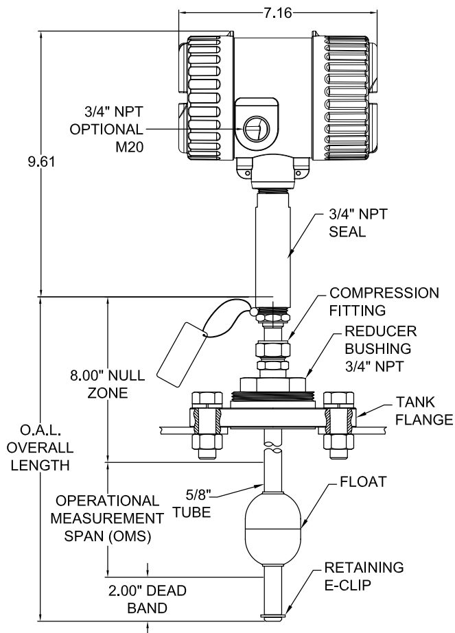
ADJUSTABLE MOUNT
