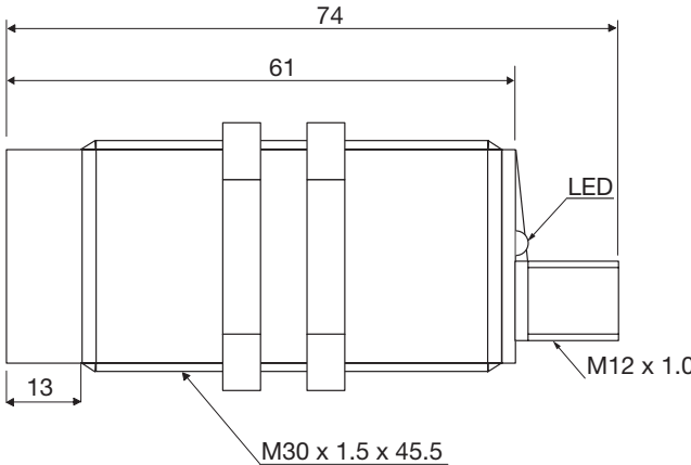
Fig. 9 Stik CA30CAN...M1IO
