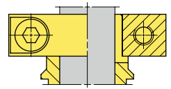
Clamping ring
