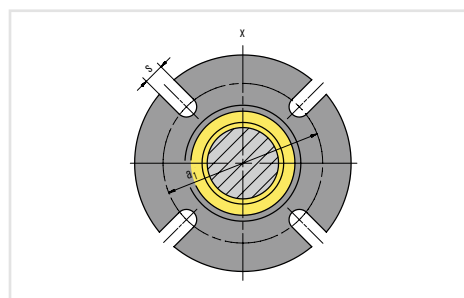
Seal flange
