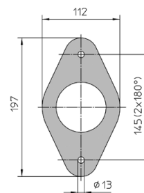
CENTA TB 1
