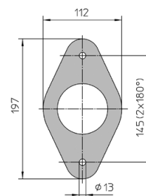
CENTA TB 1
