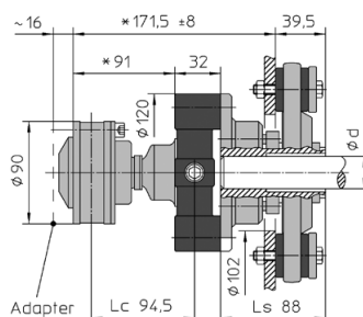
CF-ACV-8-05-1
