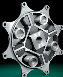
CENTAFLEX-DS
