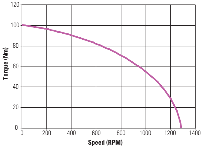
KBM(S)-88X00 ContinuousTorque
