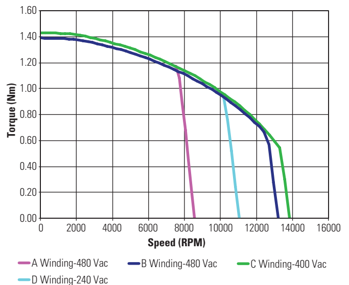
KBM(S)-10X04 ContinuousTorque
