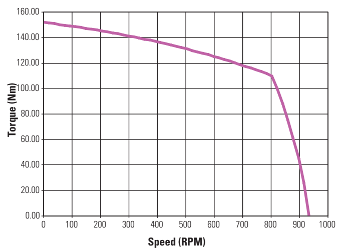
KBM(S)-60X03 ContinuousTorque
