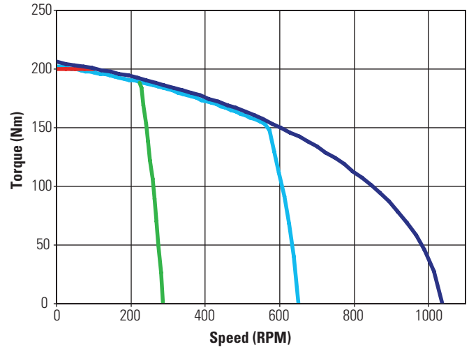
KBM(S)-88X01 ContinuousTorque
