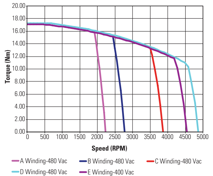
KBM(S)-35X02 ContinuousTorque
