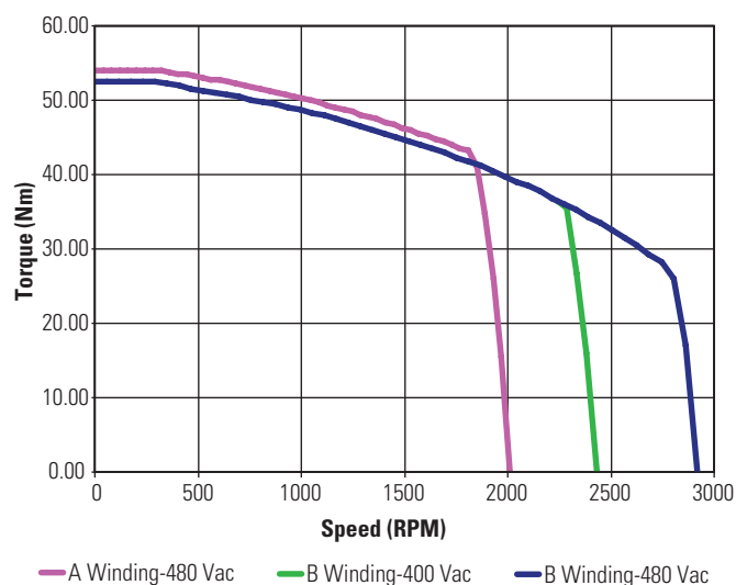
KBM(S)-45X03 ContinuousTorque
