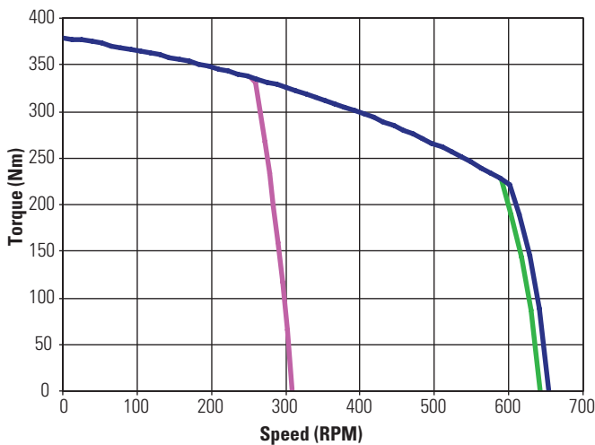
KBM(S)-88X02 ContinuousTorque
