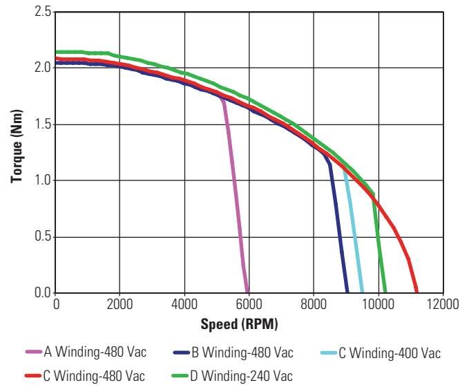
KBM(S)-14X02 Continuous Torque
