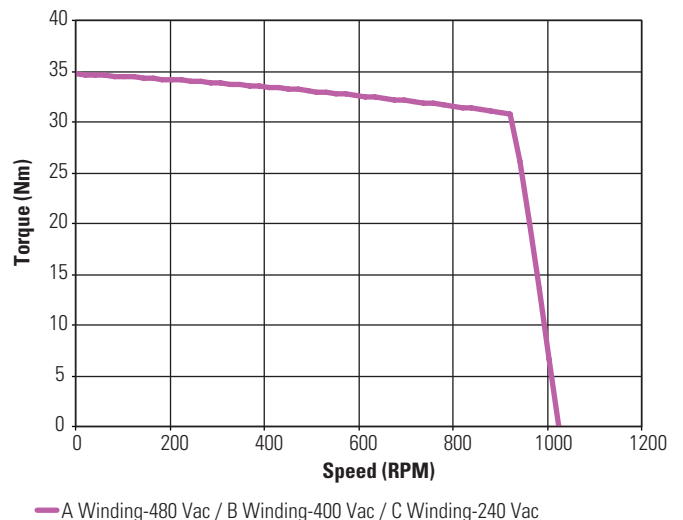
KBM(S)-43X04 ContinuousTorque
