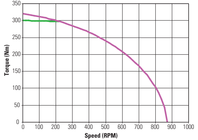
KBM(S)-118X01 ContinuousTorque
