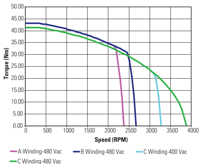
KBM(S)-45X02 ContinuousTorque
