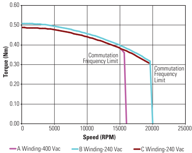
KBM(S)-10X01 ContinuousTorque
