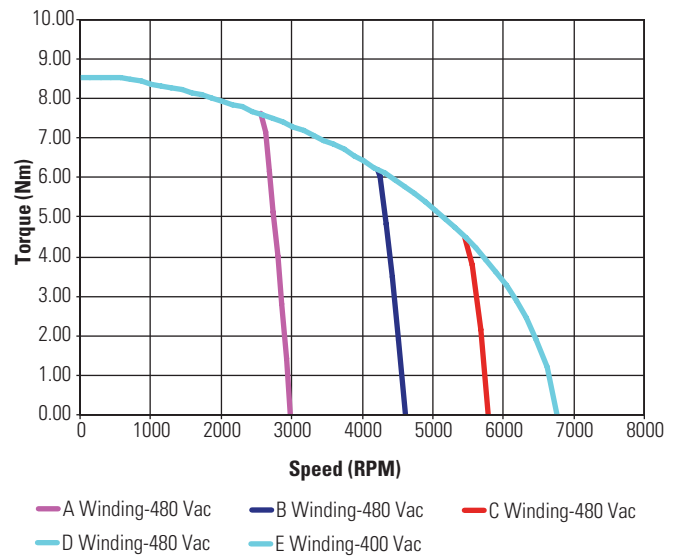
KBM(S)-25X02 ContinuousTorque
