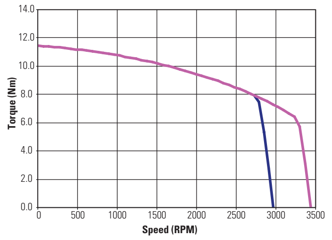
KBM(S)-43X02 ContinuousTorque
