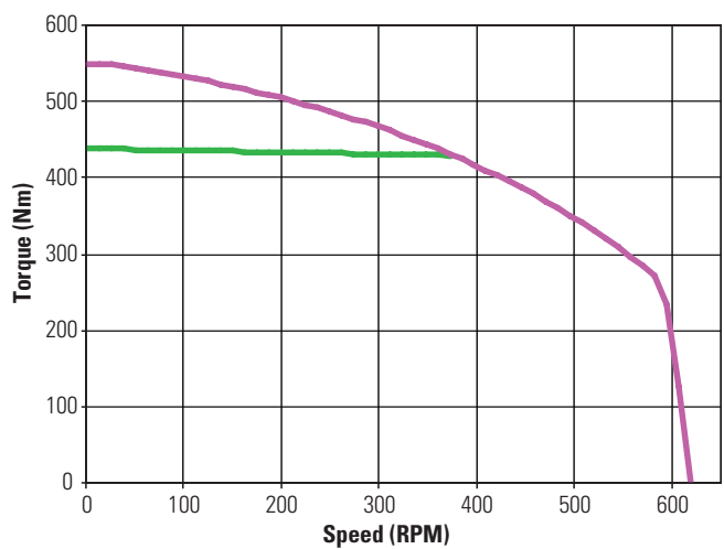
KBM(S)-118X03 ContinuousTorque
