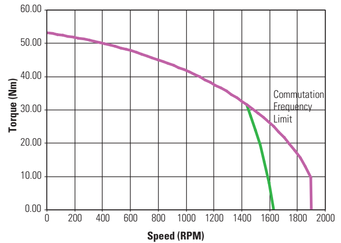
KBM(S)-60X01 ContinuousTorque
