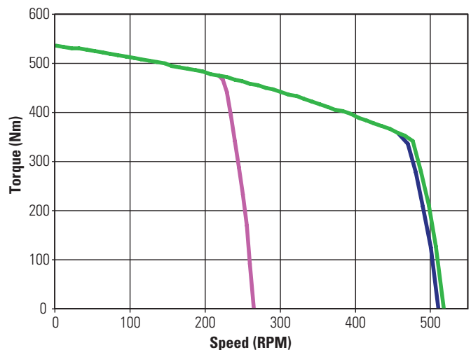
KBM(S)-88X03 ContinuousTorque
