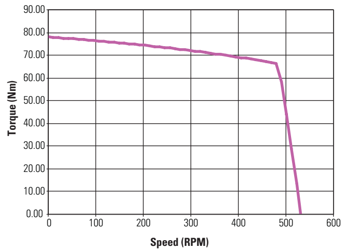
KBM(S)-79X02 ContinuousTorque
