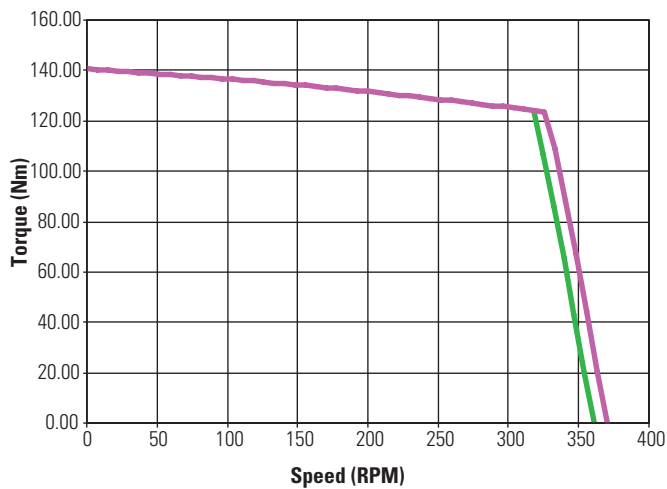
KBM(S)-79X03 ContinuousTorque
