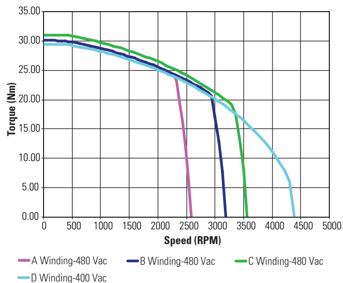
KBM(S)-45X01 ContinuousTorque
