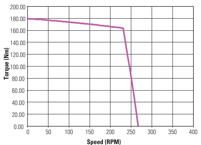
KBM(S)-79X04 ContinuousTorque
