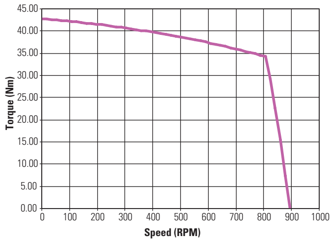
KBM(S)-79X01 ContinuousTorque
