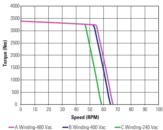
KBM(S)-260X03 ContinuousTorque
