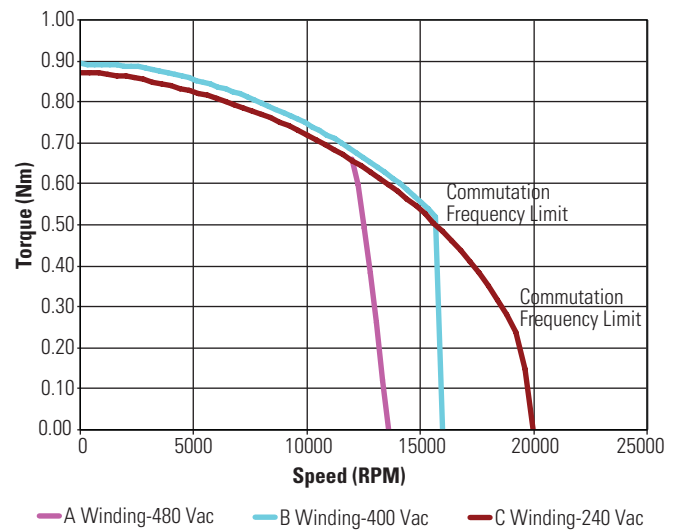
KBM(S)-10X02 ContinuousTorque
