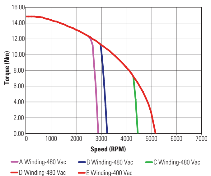
KBM(S)-25X04 ContinuousTorque
