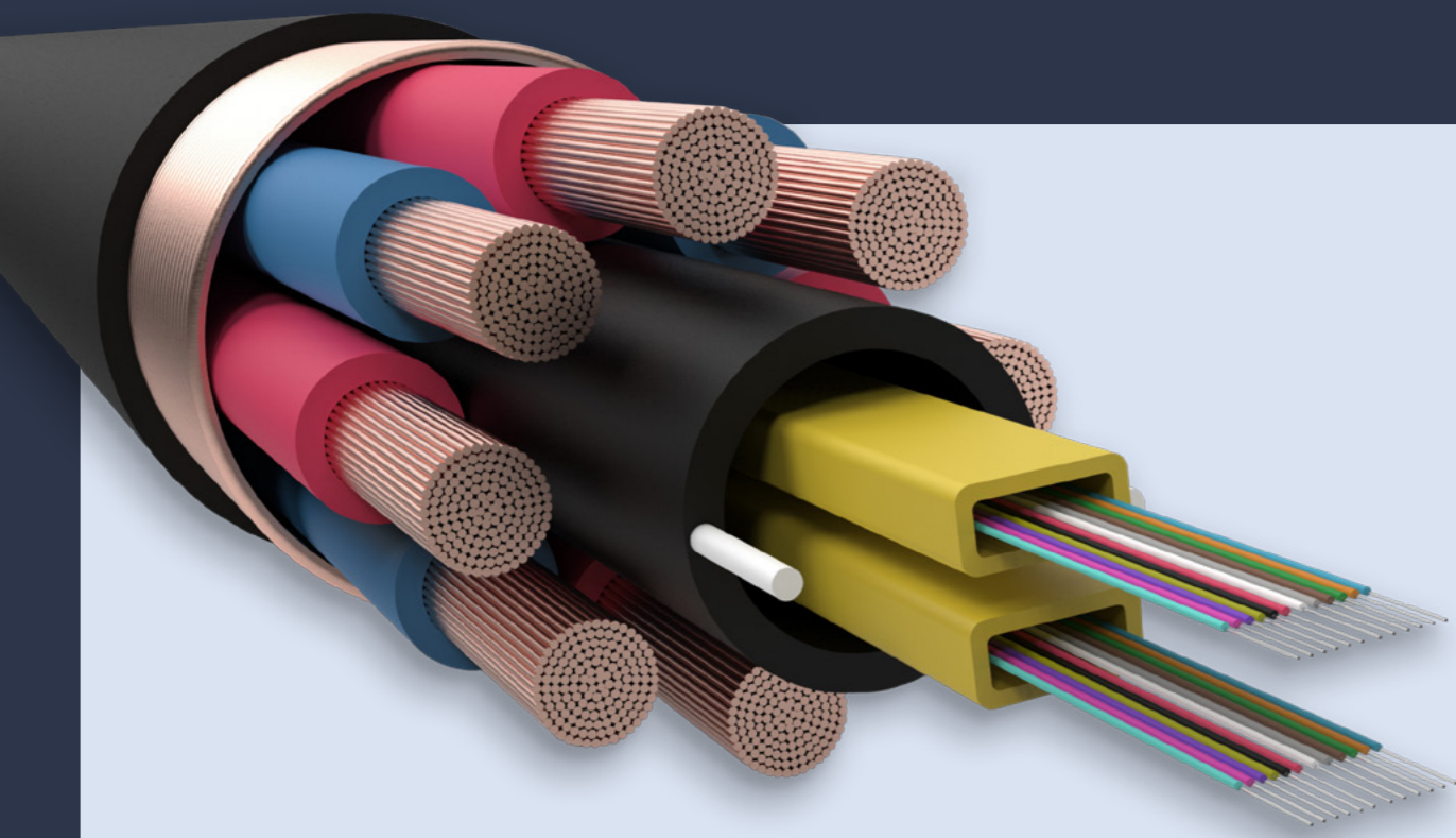
Figure 5: FTTH 48 VDC hybrid cable 8 × 10 mm 2 cores and 24 SM fibres
