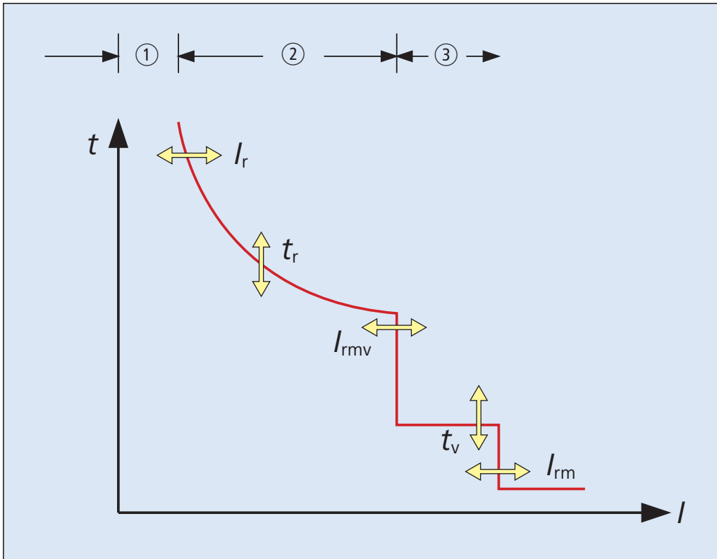
Figure 5: The figure indicates a tripping characteristic with functional ranges 1. Non-trip range / operating range to the left of or under the red tripping characteristic, 2. Overload range, a brief overload is possible, 3. Short-circuit range. The figure also indicates the variable parameters corresponding to Table 4, which enable application-specific design of the characteristic curve.
