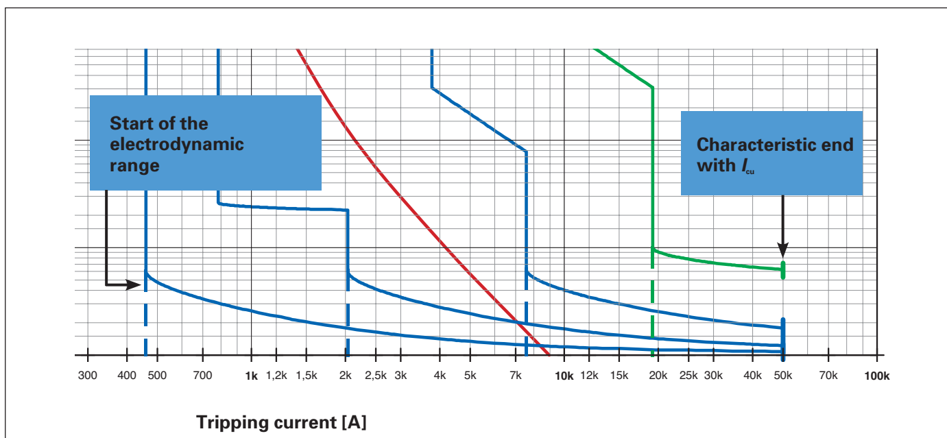
Figure 7: On the lower end range of the curves, a dynamic behaviour of the switch cannot be calculated with a reasonable amount of effort. For a binding statement regarding selectivity in this range, you are referred to the test results in the selectivity table in the Eaton main catalogue Industrial Switchgear.
