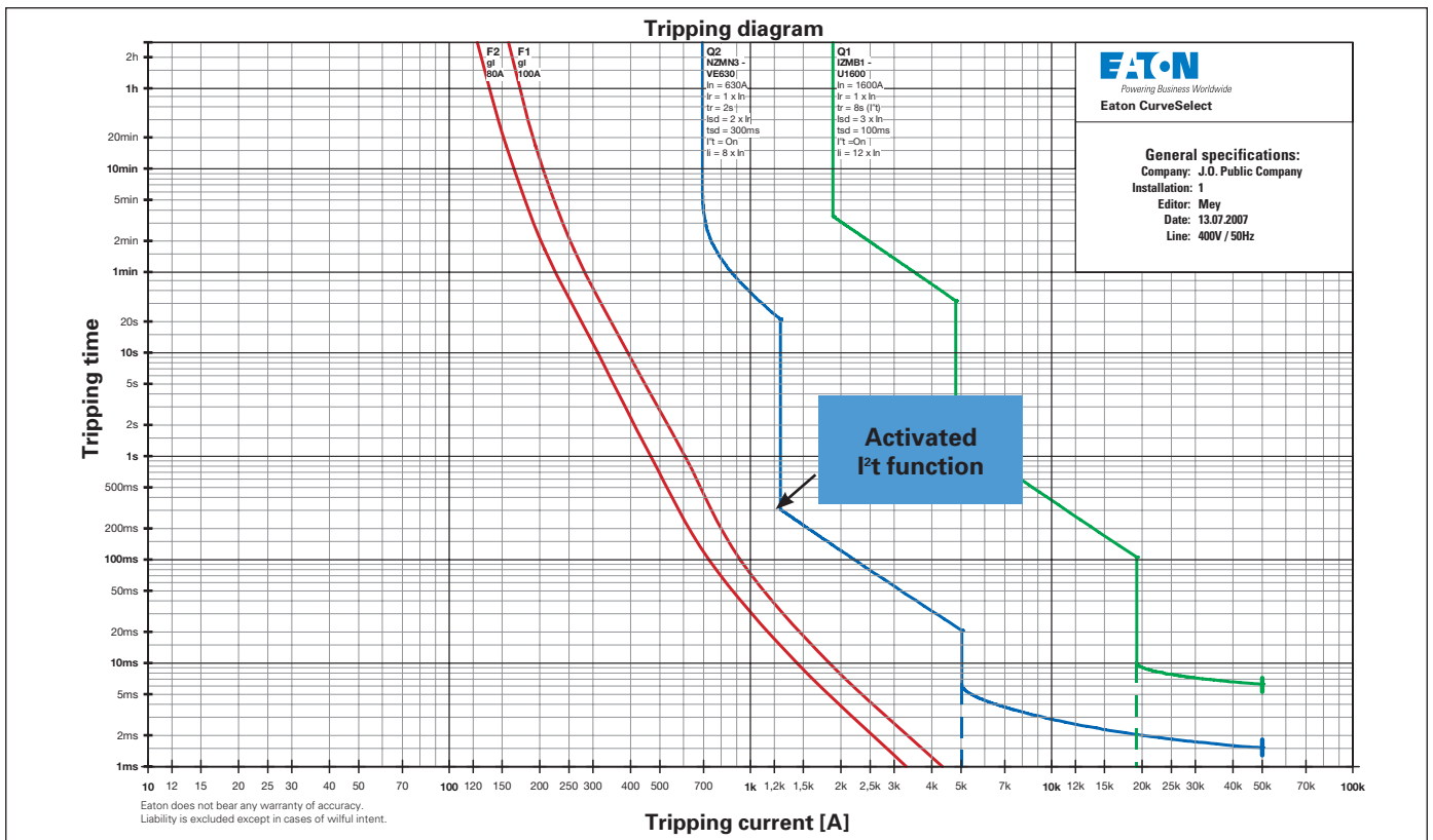
Figure 9: In contrast to Figure 8, the circuit-breaker represented in blue has been reselected. The modified settings provide selectivity in the overload and short-circuit range. The selectivity which is evident in the short-circuit range is confirmed by the selectivity specifications in the main catalogue Industrial Switchgear. The I^2t function can be switched on and off. It improves the selectivity with fuses.
