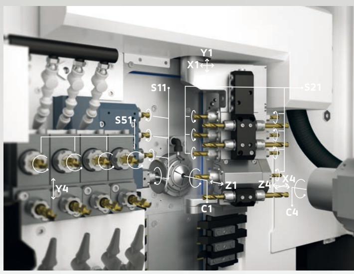
Swiss GT 26B & Swiss GT 32B
