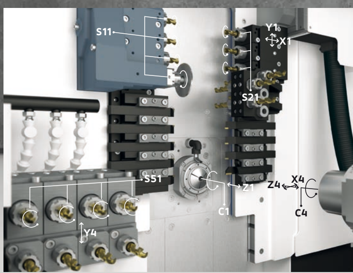
Swiss GT 26 & Swiss GT 32
