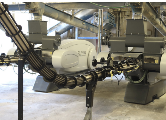
Two BP5510 Briquetting Presses producing industrial briquettes from sawdust.
