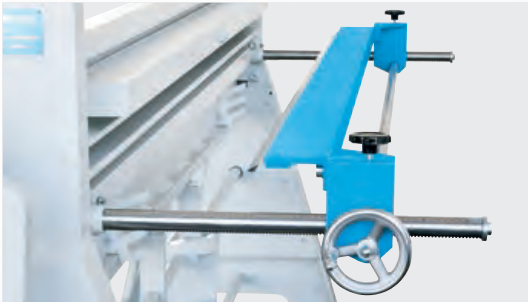
1 BACK GAUGE WITH STOP BAR
