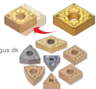
ECOTURN Regular size CNMG090408E type CNMG120408 type
