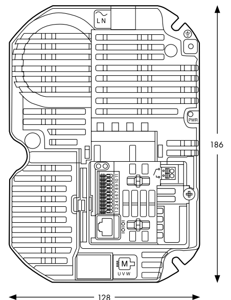
PFC drive
