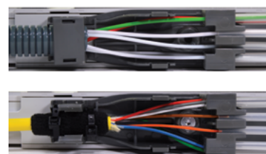
Figure 21: Installed FACT-ACCCTULLT
