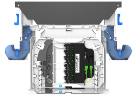
Figure 15: Right cable exit MPO module with LC/APC ports
