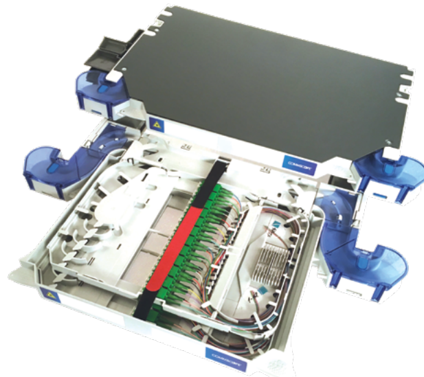
Figure 1: FACT splice-patch chassis
