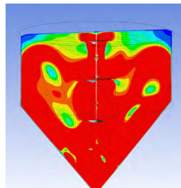
A simulation of an agitator in a large digester shows even flow that guarantees good temperature distribution and high gas production.
