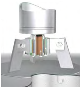
Bottom bearing
