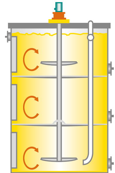
Recausticizing tank
