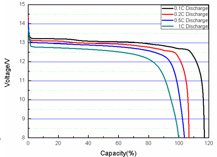
Discharge performance
