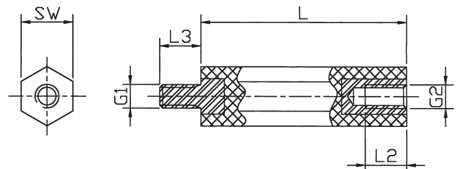
HEXAGON SHAPE: EXECUTION DIA [ Internal / external thread ]
