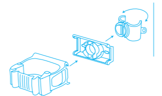
Toolflex One Motion includes Toolflex One holder, adapter and tube clamp.
