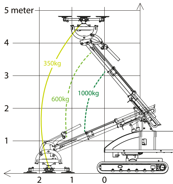
LASTDIAGRAM - VANDRETTE SUGEKOPPER
