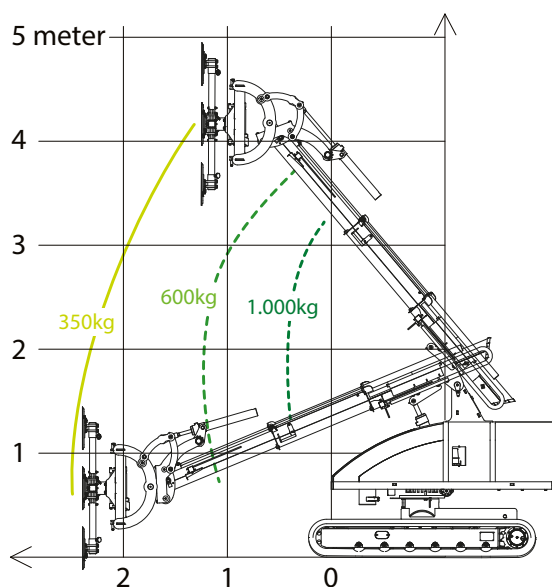
LASTDIAGRAM - LODRETTE SUGEKOPPER
