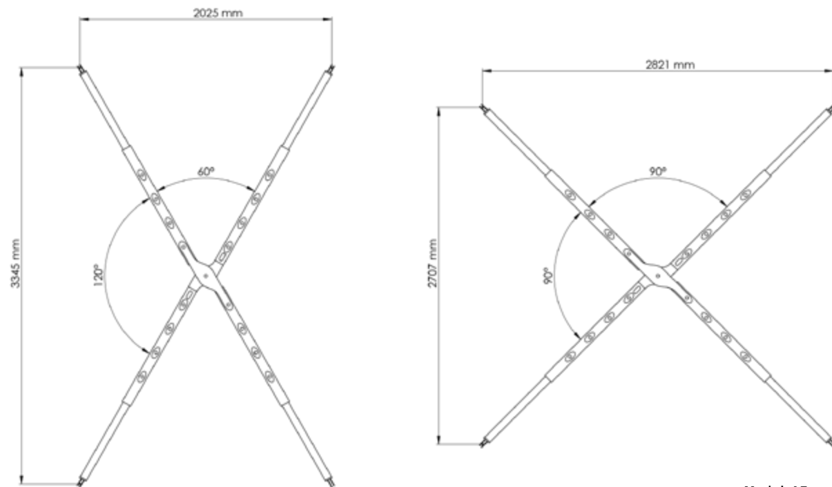
Model: A5 Max load: 5 ton Material: Aluminium
